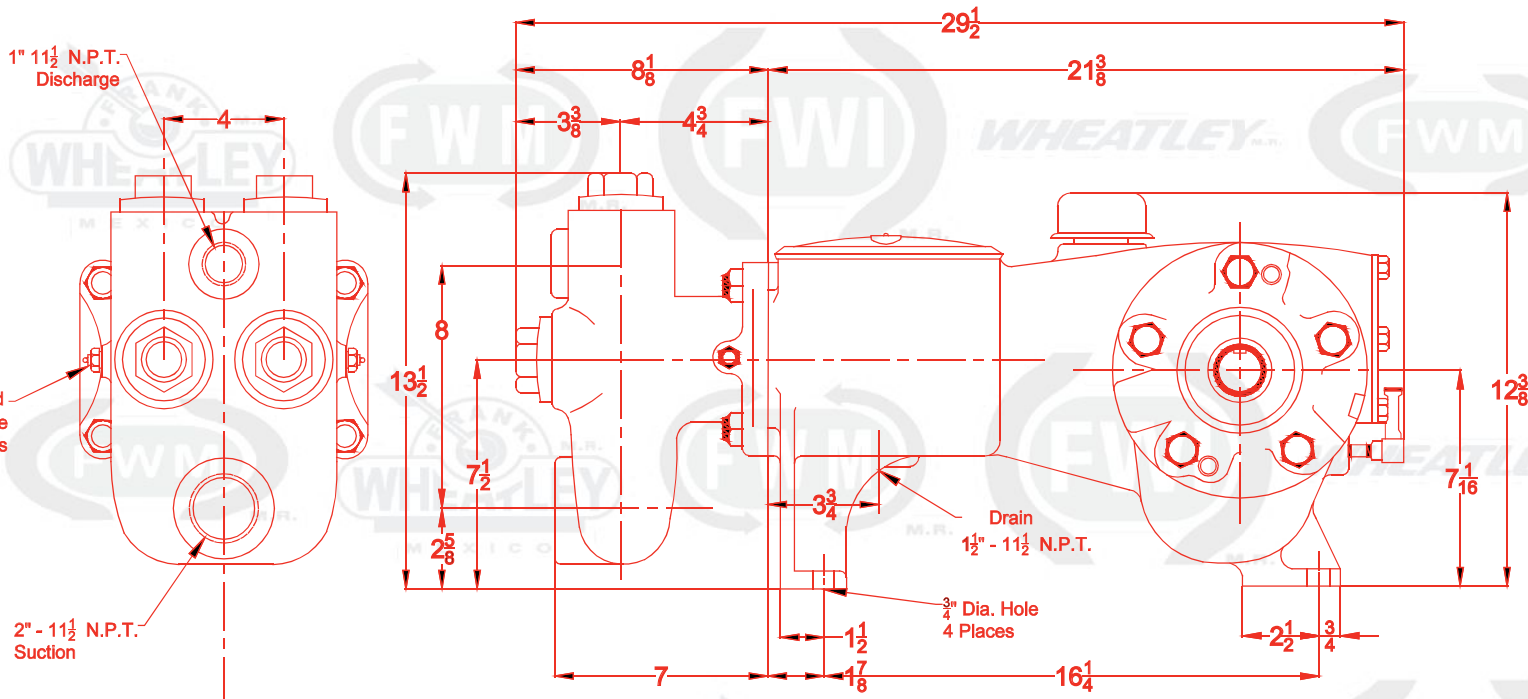
CAST ALUMINUM BRONZE OR DUCTILE IRON FLUID CYLINDER
